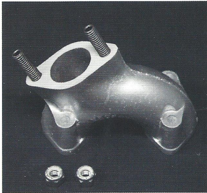
Side Manifold for Triumph
